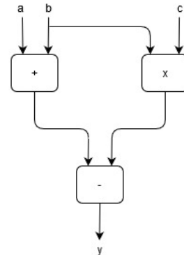
Figure 3: Simple Data-Flow Model of y = (a + b) - (b * c)
